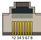
8-position 8-contact (RJ-45)
