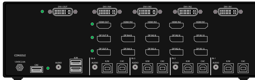
Figure 4-2: KVS4-1004VMX Rear panel
