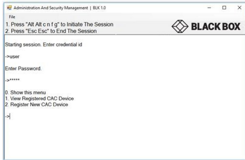
Figure 3: User Log-in
