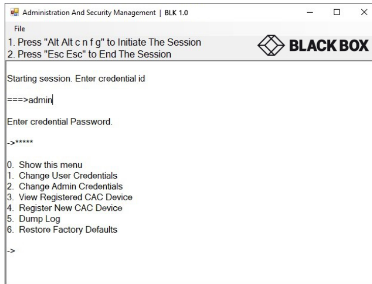
Figure 7: Administrator Log-in
