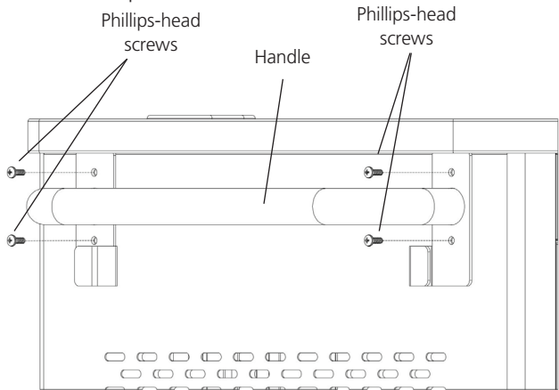
Figure 4-1. Handle assembly.
