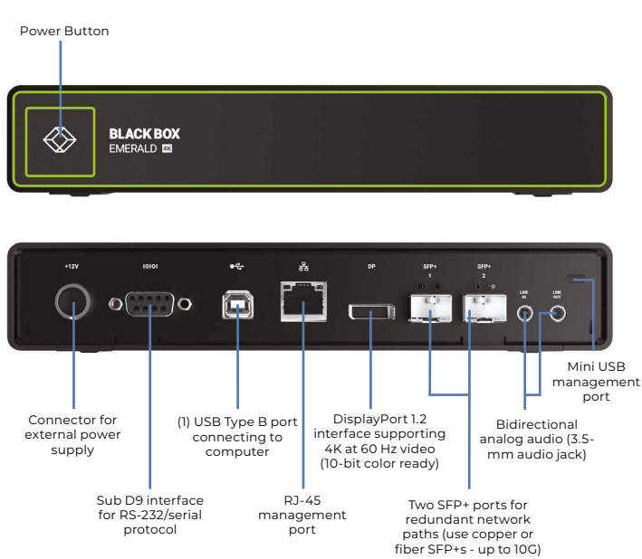
Emerald 4K Transmitter (EMD4000T)
