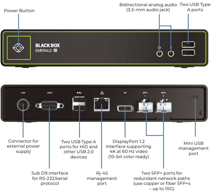
Emerald 4K Receiver (EMD4000R)
