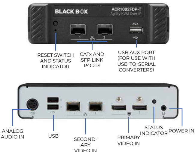
Agility Dual Monitor DisplayPort Transmitter (ACR1002DP-T)
