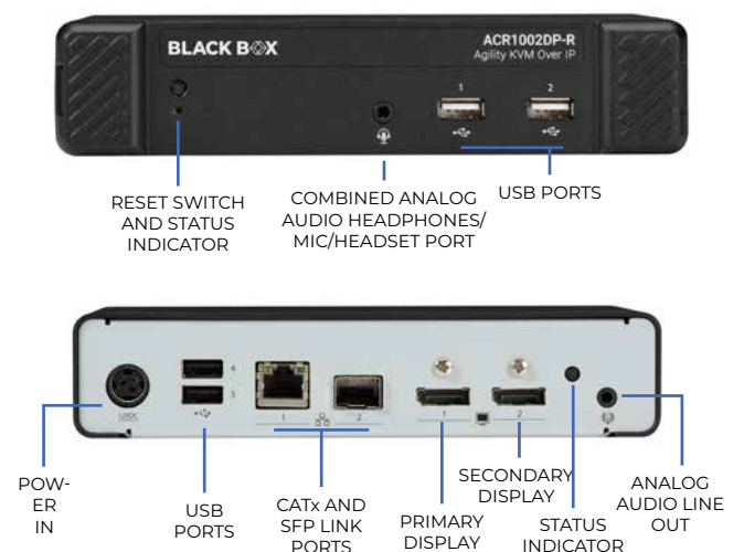
Agility Dual Monitor DisplayPort Receiver (ACR1002DP-R)
