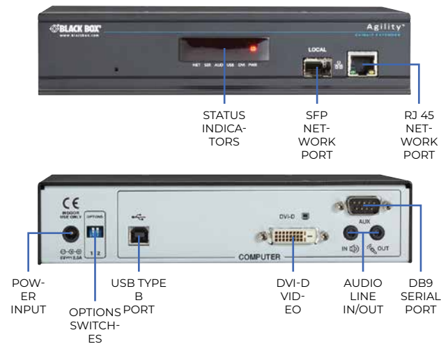
Agility Single Head DVI Transmitter (ACR1000A-T-R2)
